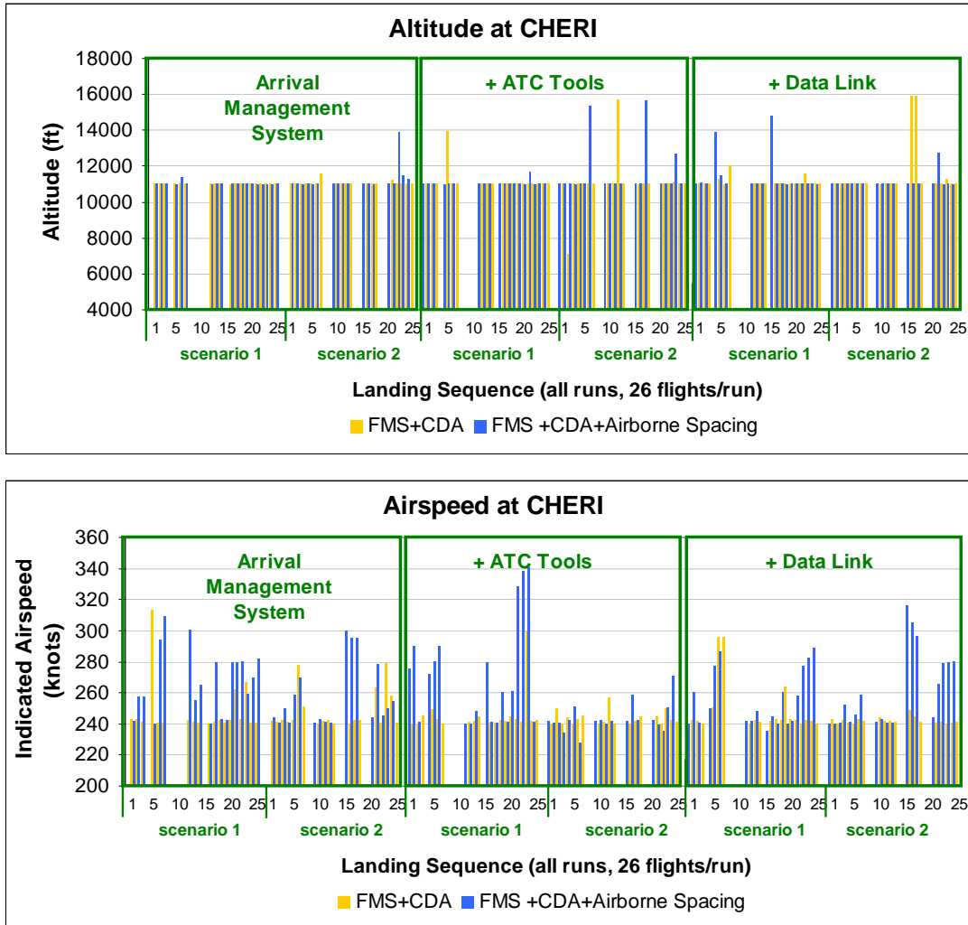
Figure 15: Crossing altitude and speed at CHERI
