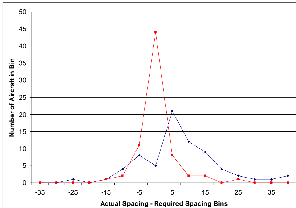
Figure 13: Spacing error at the runway.
