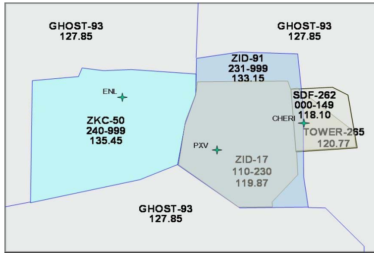
Figure 5: Sector map of test airspace
