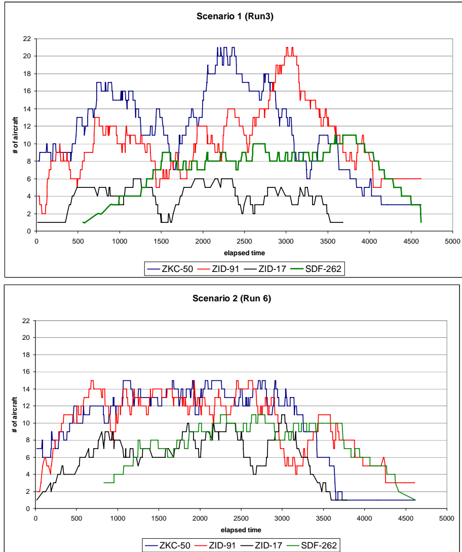
Figure 10: Traffic loads for the two scenarios
