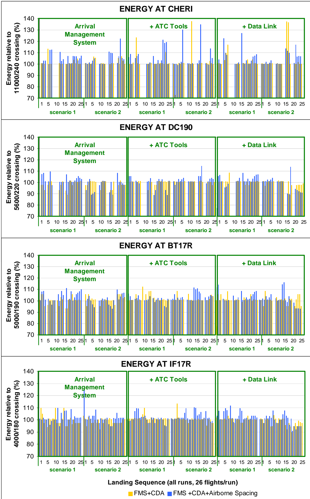
Figure 16: Relative energy along the CHERI CDA
