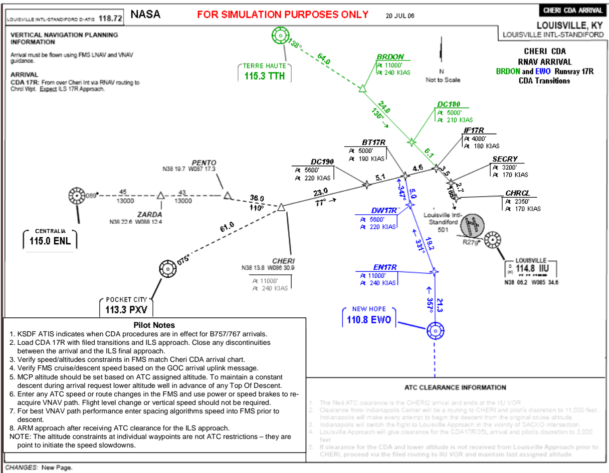
Figure 4: Continuous Descent Approach (CDA) used during simulation
