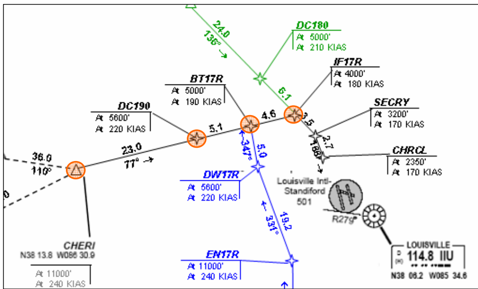
Figure 14: altitude and speed at CHERI
