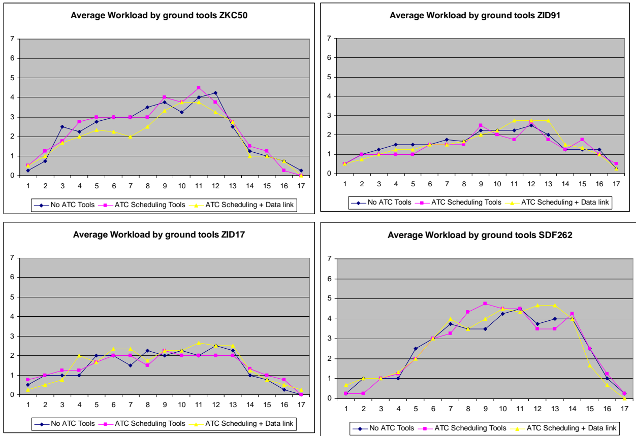
Figure 11: Average controller workload by ATC condition
