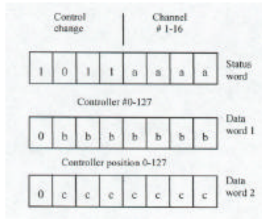
Figure 5.5. Anatomy of a MIDI control change message for transmitting data from continuous controllers. In this case, the controller number is mapped to a particular function on the MIDI device (e.g., azimuth control input), while the position is mapped to the value for that particular function (e.g., where on the azimuth).
