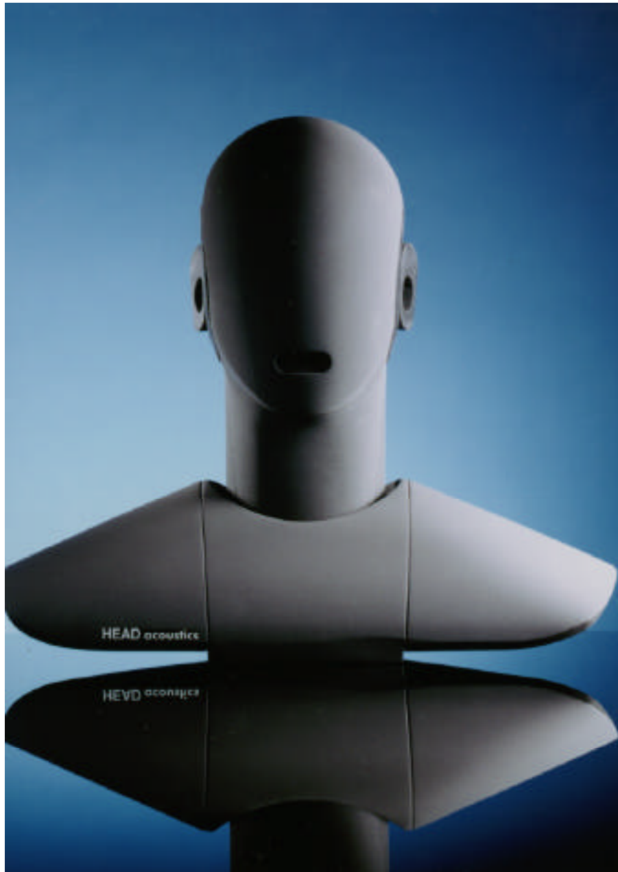
Figure 4.27. The AACHEN Head Model HMS II, manufactured by HEAD acoustics. The outer ears are designed according to a “structural averaging” of HRTFs; note the inclusion of the upper torso. Two versions of the head are available: the HMS II, intended for analysis within an integrated system, and the HRS II, for recording studio applications. Photograph courtesy of Wade Bray, Sonic Perceptions–HEAD acoustics.
