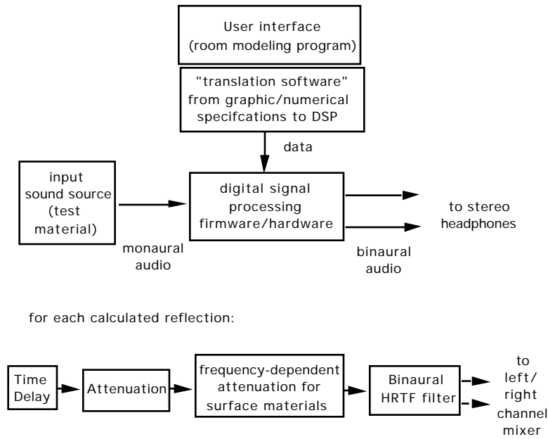
Figure 4.53. The basic components of a signal processing system used in an auralization system.
