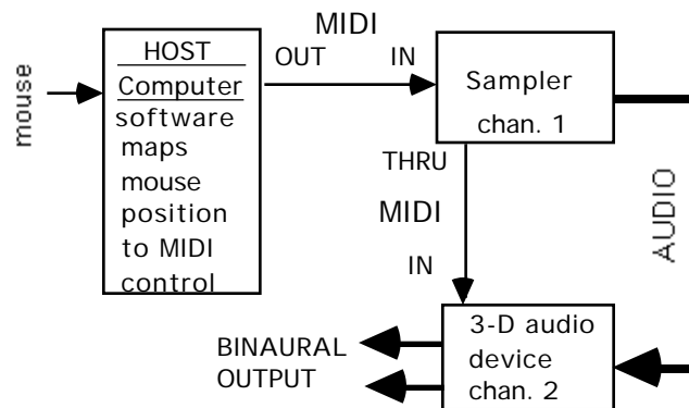
Figure 5.3 Illustration of the control signal paths for a mouse–audio interface showing how multiple devices can be addressed by MIDI control signals. Tracing the audio signal paths, a monaural signal is generated by the sampler, and is then spatialized into a two-channel binaural output by the distributed 3-D audio device for output to stereo headphones. Tracing the control signal paths, the computer is used as a MIDI controller and the sampler and 3-D audio devices act as MIDI slaves. The slaves are connected in series, but can be addressed independently due to their unique MIDI channel number. The mouse position is read as control signals to the host computer’s operating system; a software program reinterprets this into commands that are sent out the computer’s MIDI out port to the MIDI in port of the sampler, which responds to information addressed to MIDI channel 1. The MIDI thru port of the sampler passes instructions from the computer unchanged to the MIDI in port of the 3-D audio device, which is set to respond only to MIDI channel 2.
