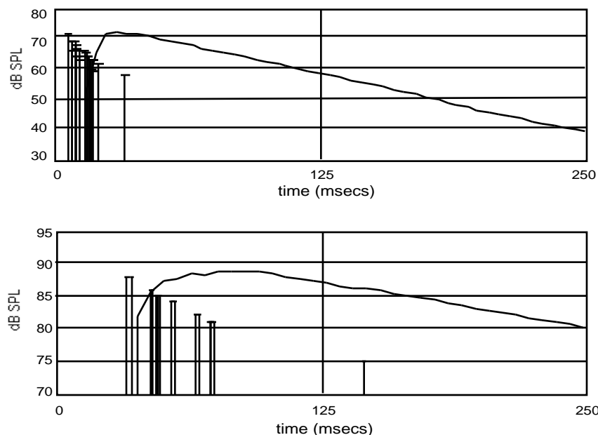
Figure 3.15. Reverberant decay and early reflections in (top) a small room 2 feet from a sound source, and (bottom) in a very large room, 30 feet from a sound source. Note that in the larger room the early reflections are masked by the reverberant decay and that the rate of decay is much slower than in the smaller room (7 dB between 125–250 msec, as opposed to 19 dB). Graphic adapted from Modeler® room design program, Courtesy of Bose® Corporation.
