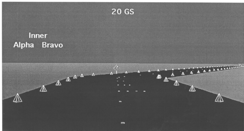
Figure 2. Depiction of HUD taxi symbology over a generic taxiway. All HUD symbology shown in white (actually green).
