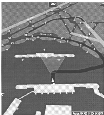
Figure 1. Electronic Moving Map, showing the ownship about to proceed from Concourse B and follow a cleared route to Runway 9L at Chicago O'Hare. The triangle represented the center of gravity of the ownship, and the light triangular area in front represented the pilot's actual visual field (i.e., the area visible out the window). Route guidance was provided by the darkened area (actually magenta). Note the menu of zoom levels in the bottom right hand corner of the display; these were self-selectable.
